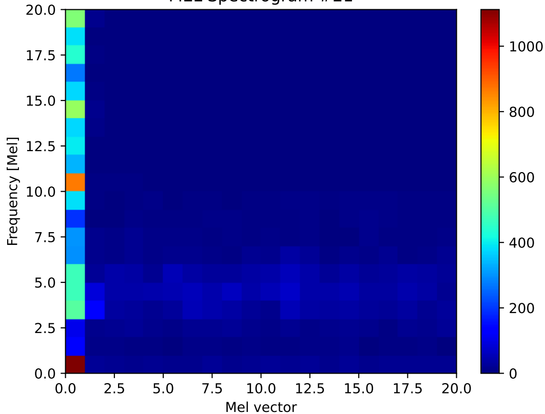
MEL Spectrogram #21
